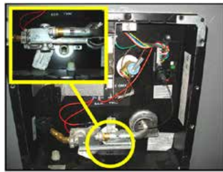
Water heater drain plug
