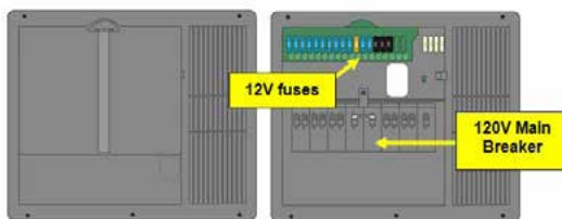
Load Center Panel w/120 volt Main Breaker (load center appearance and configuration may vary by model)
