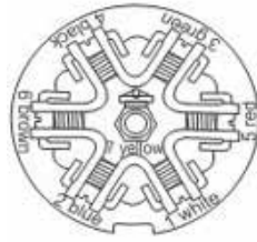
7-way trailer plug car end, rear view
