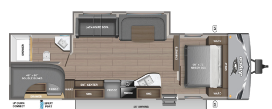
284BHS/BHSW
