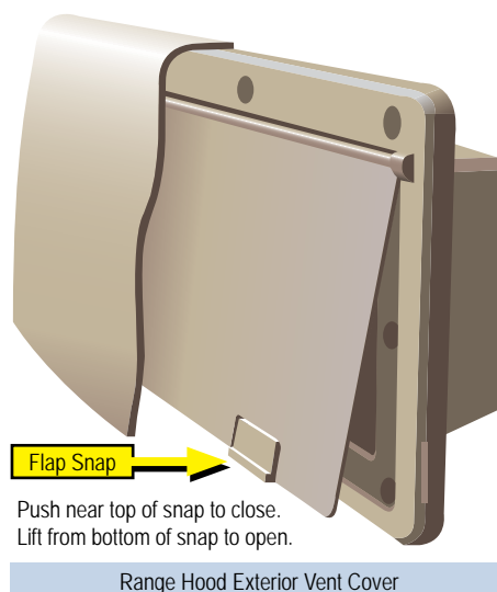
Range Hood Exterior Vent Cover
