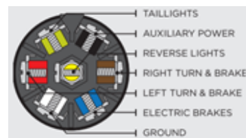
View from Trailer Wire Entry Side
