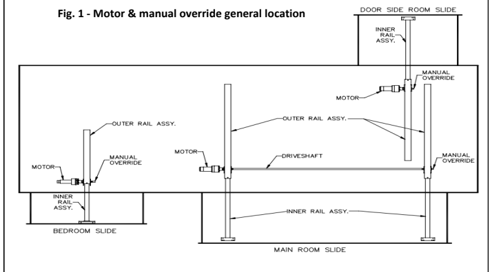
Fig. 1 - Motor & manual override general location
