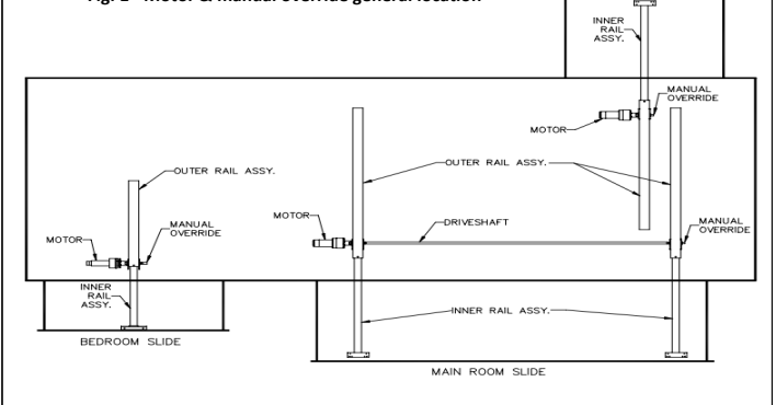
Fig. 1 - Motor & manual override general location
