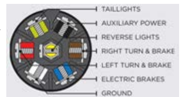
View from Trailer Wire Entry Side
