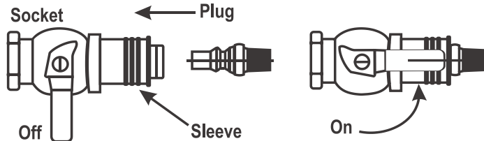
Quick Coupler Connection
