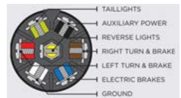
View from Trailer Wire Entry Side
