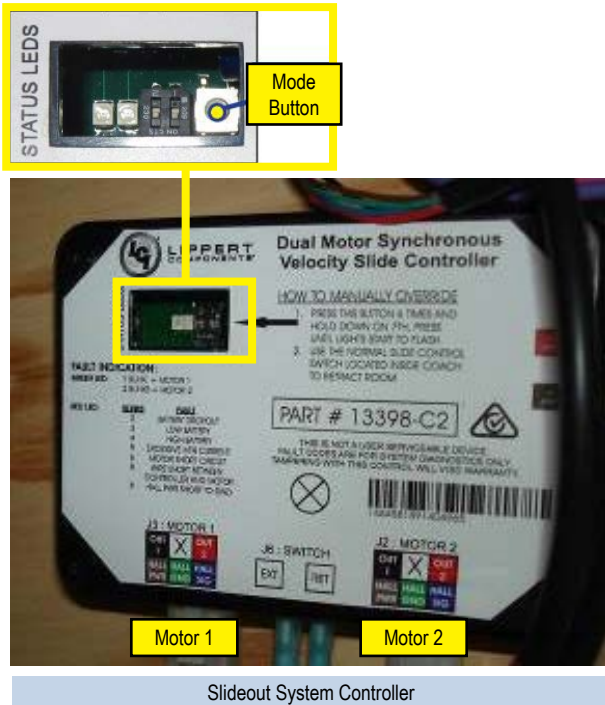
Slideout System Controller
